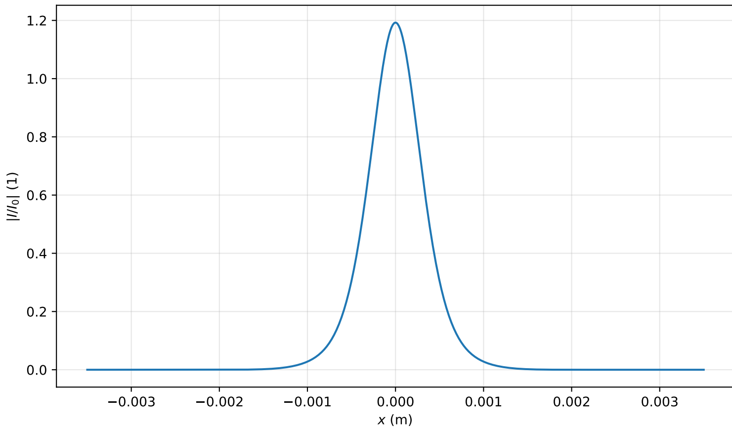
Intensity profile I(x, y = 0, z = 1.513m)/I_0 , P_{in}=0.7P_{cr} , artificial time
